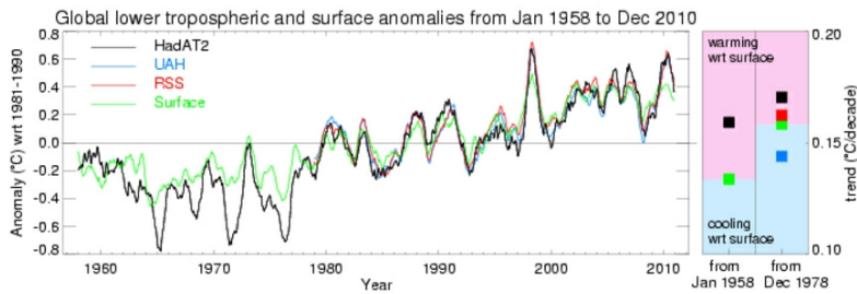
Figure 1: HadAT2 radiosonde data (black) vs. UAH (blue) and RSS (red) lower troposphere temperatures, and HadCRUT3 surface temperatures (green)
