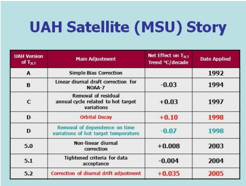
Figure 2: Major corrections to the UAH temperature trend over the years.
