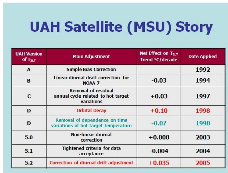
Figure 2: Major corrections to the UAH temperature trend over the years.
